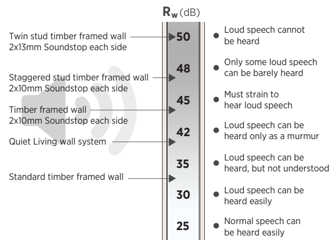
Figure 4: Noise Levels
