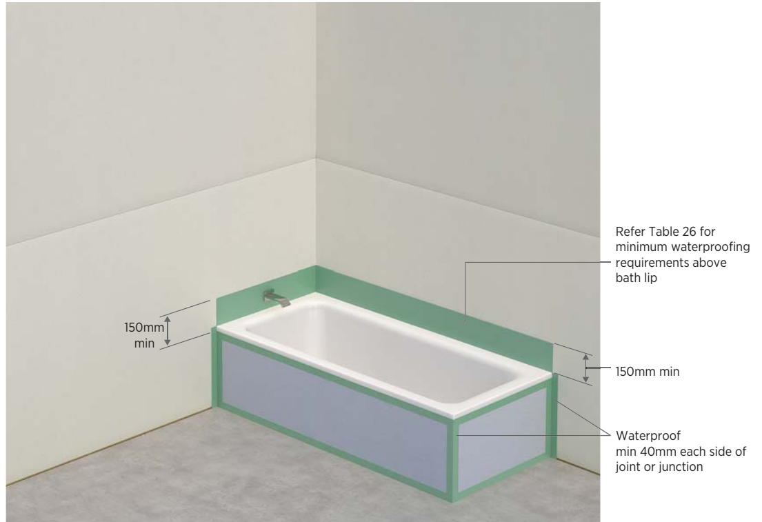
Figure 57: Waterproofing of bath
