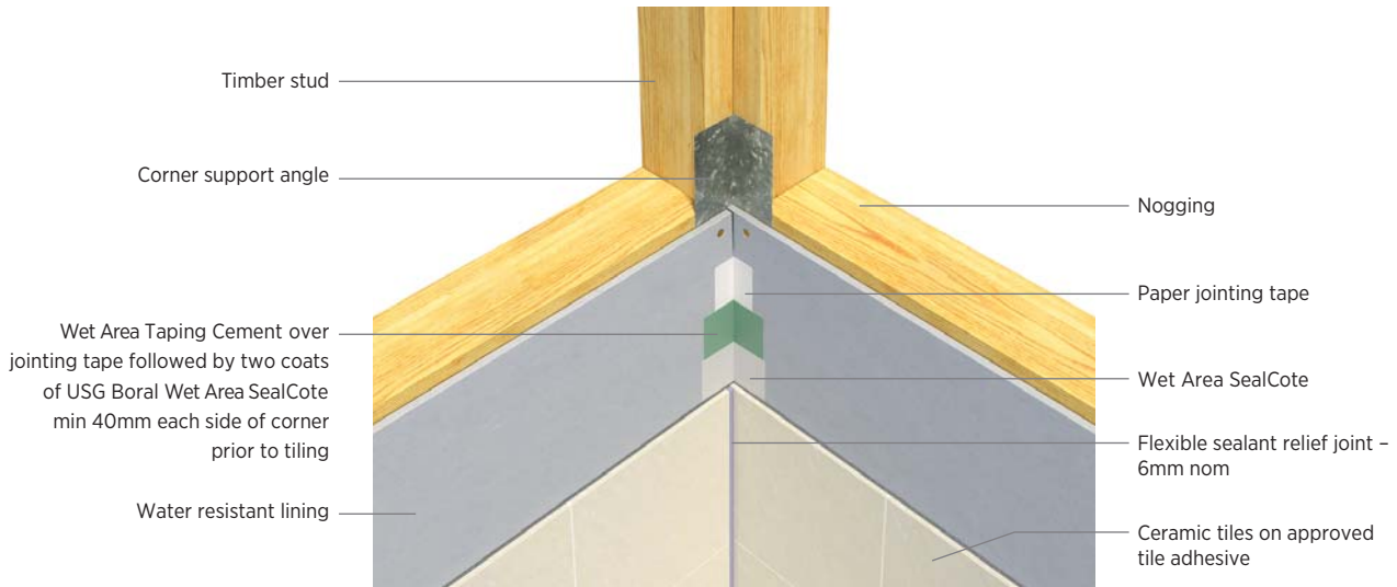
Figure 63: Internal Corner
