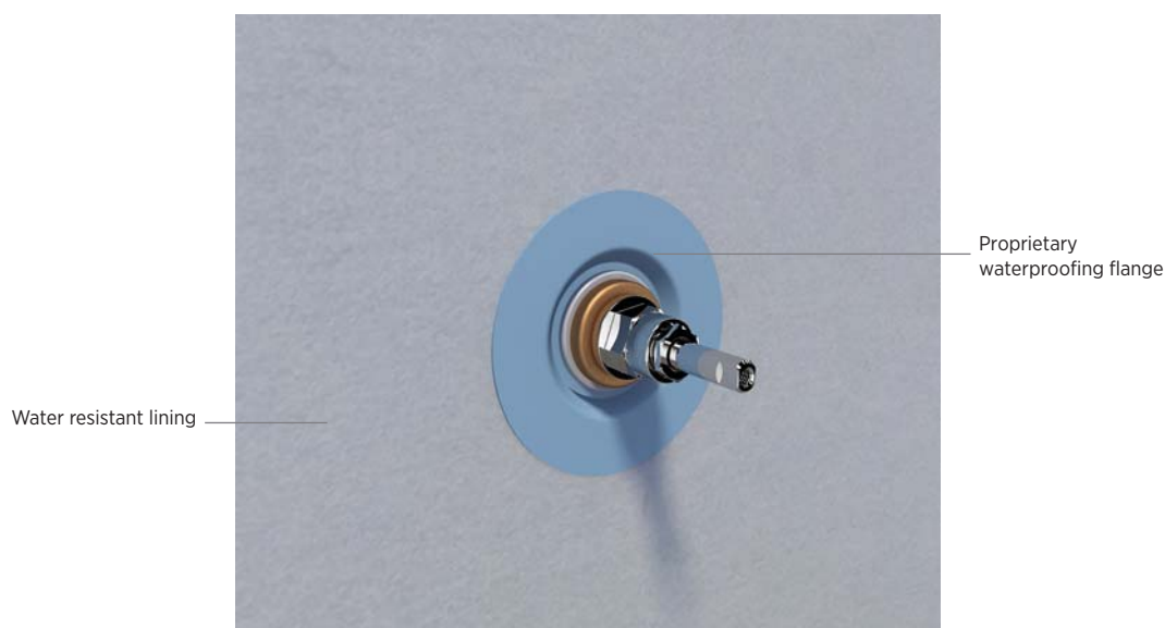
Figure 70: Plumbing Penetrations With Proprietary Waterproofing Components
